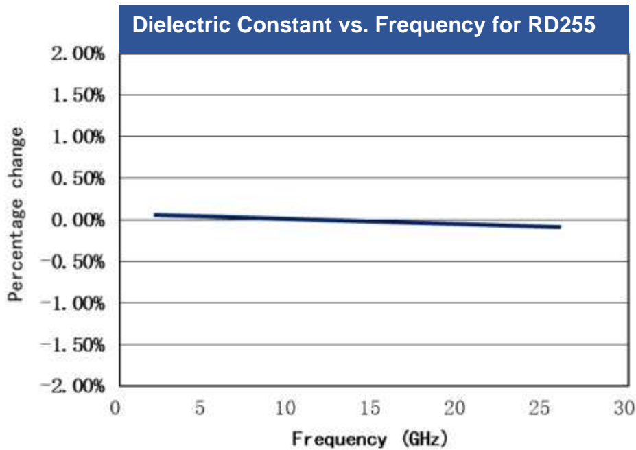
Figure 1 Demonstrates the Stability of Dielectric Constant across Frequency. The stability of the Dielectric Constant of RD255 at different frequencies simplifies design and ensures good transition and scalability of design.
